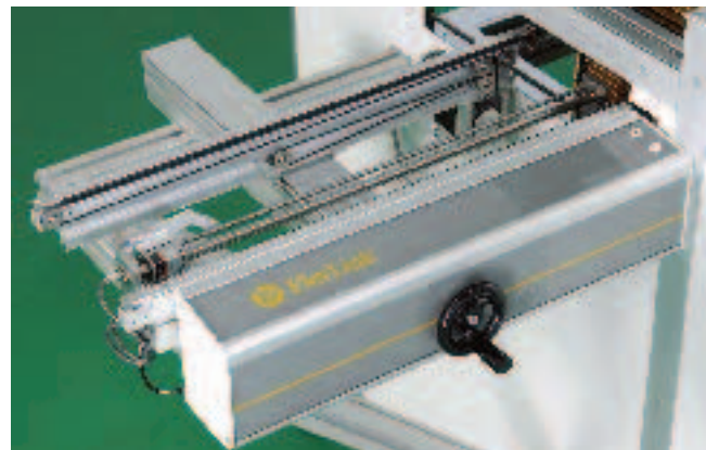
Infeed platform with "break-away" pusher
